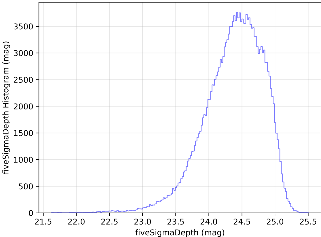
extra_ss_neo5_v3.4_10yrs g: fiveSigmaDepth Histogram
