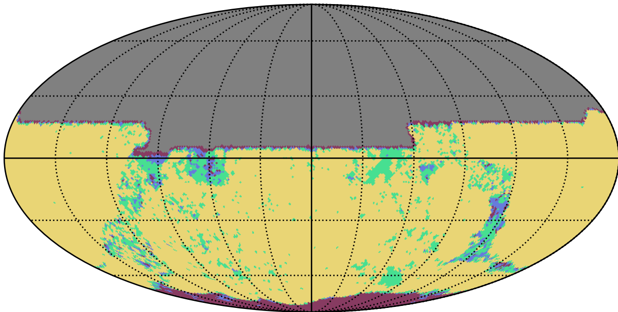
extra_ss_neo5_v3.4_10yrs y band: YearCoverage night
