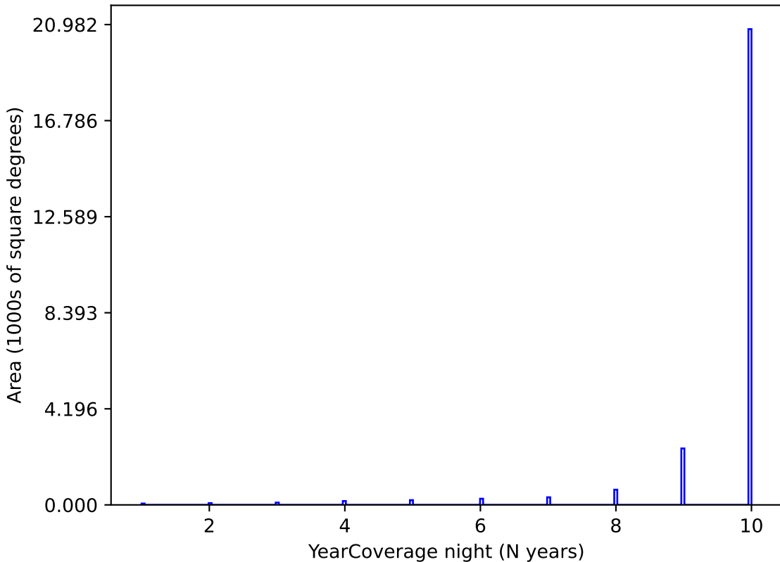
extra_ss_neo5_v3.4_10yrs y band: YearCoverage night
