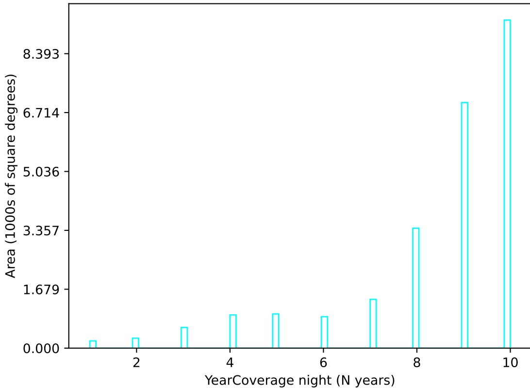
extra_ss_neo5_v3.4_10yrs u band: YearCoverage night
