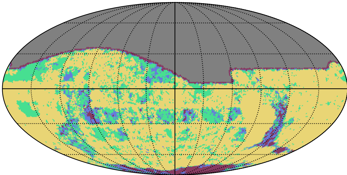
extra_ss_neo5_v3.4_10yrs g band: YearCoverage night
