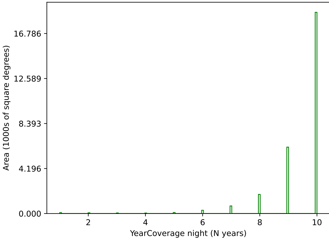
extra_ss_neo5_v3.4_10yrs g band: YearCoverage night
