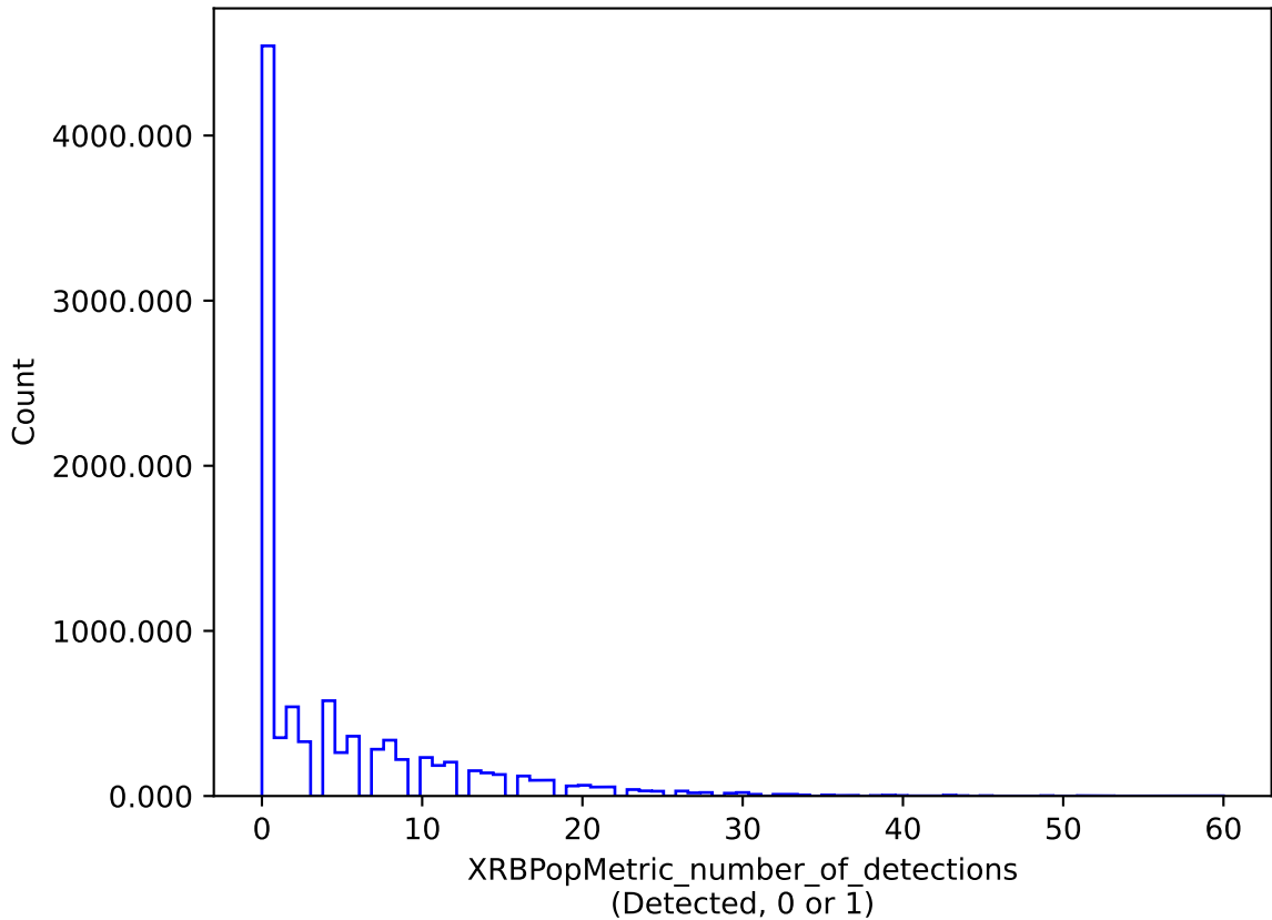
extra_ss_neo5_v3.4_10yrs : XRBPopMetric_number_of_detections
