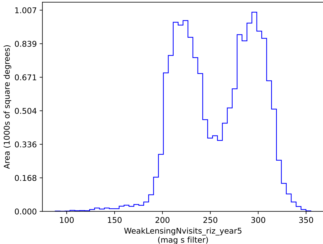
extra_ss_neo5_v3.4_10yrs gri band non-DD: WeakLensingNvisits_riz_year5
