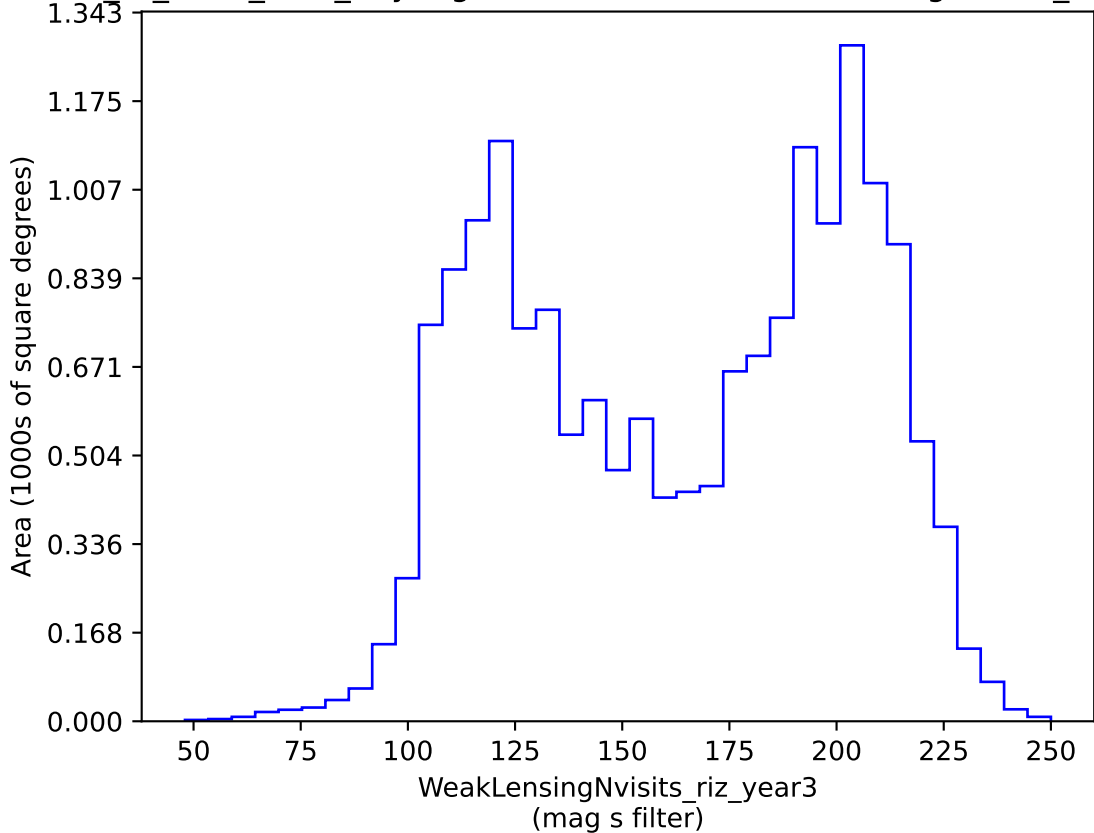
extra_ss_neo5_v3.4_10yrs gri band non-DD: WeakLensingNvisits_riz_year3
