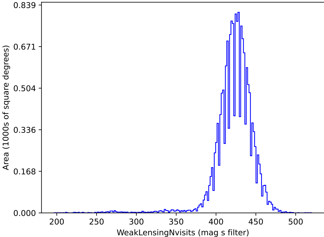
extra_ss_neo5_v3.4_10yrs gri band non-DD: WeakLensingNvisits
