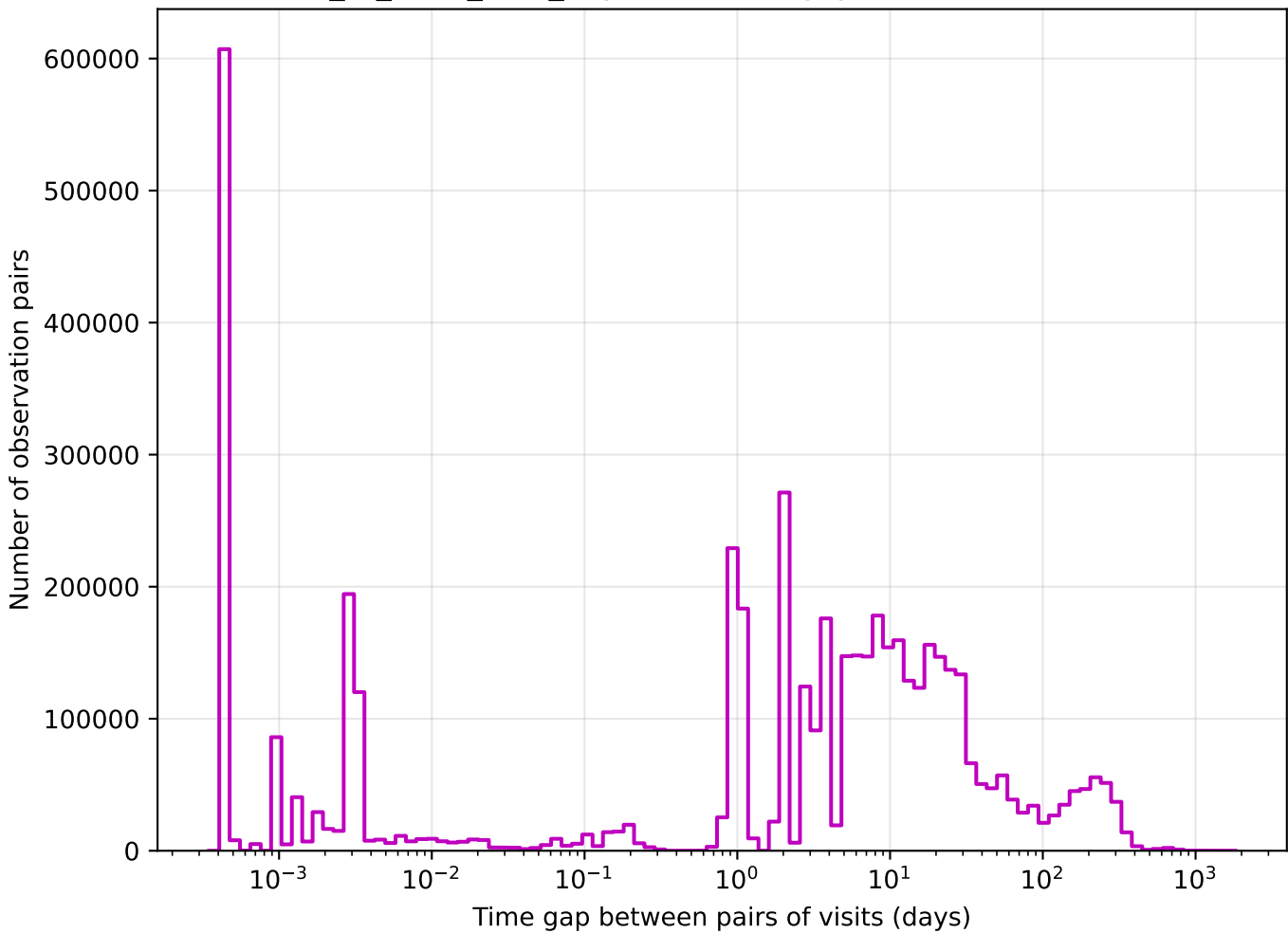
extra_ss_neo5_v3.4_10yrs z band: Tgaps observationStartMJD
