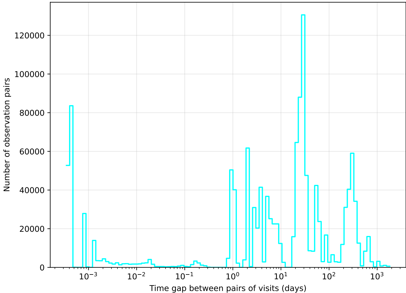
extra_ss_neo5_v3.4_10yrs u band: Tgaps observationStartMJD
