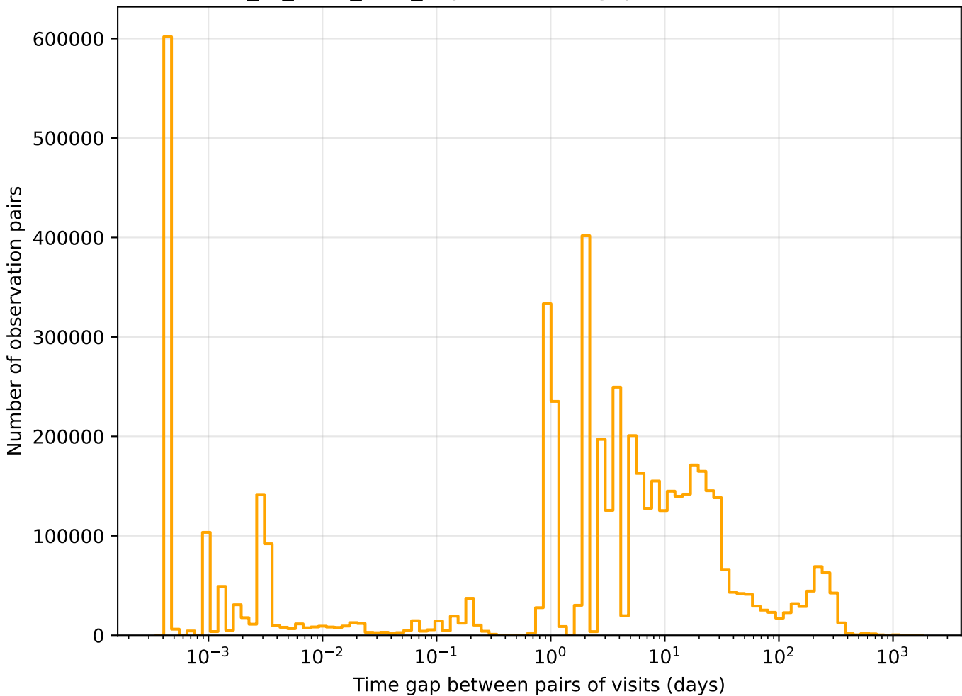
extra_ss_neo5_v3.4_10yrs r band: Tgaps observationStartMJD
