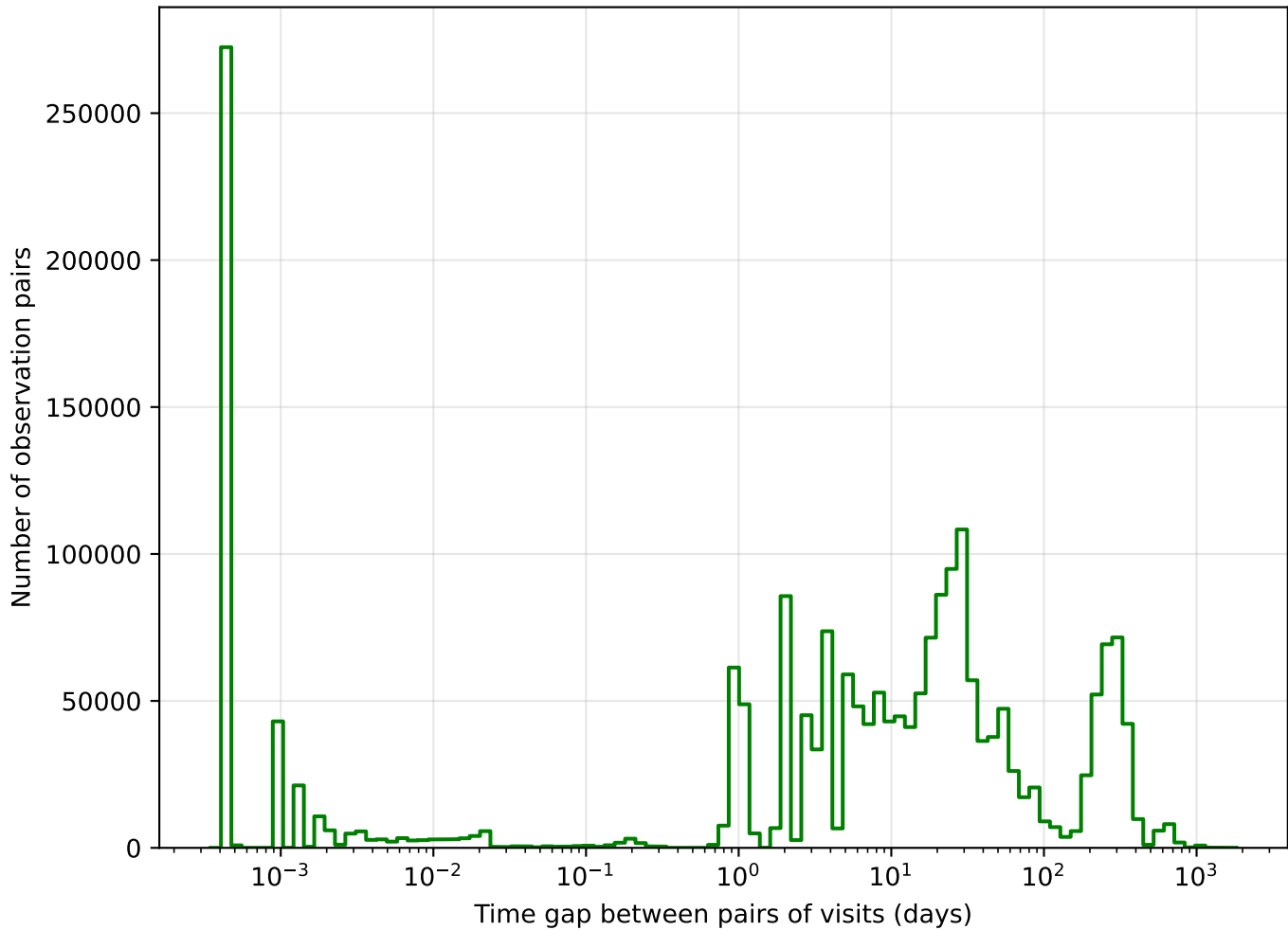
extra_ss_neo5_v3.4_10yrs g band: Tgaps observationStartMJD
