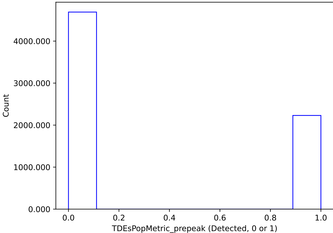
extra_ss_neo5_v3.4_10yrs : TDEsPopMetric_prepeak
