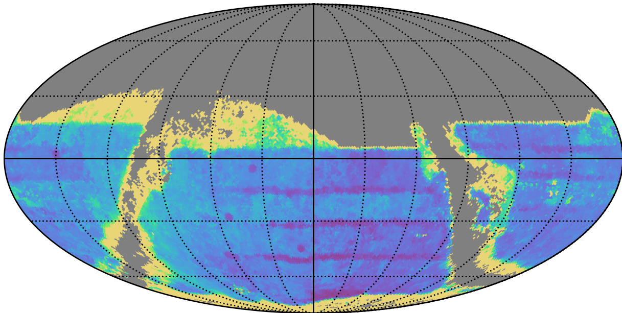
extra_ss_neo5_v3.4_10yrs : TDC_accuracy
