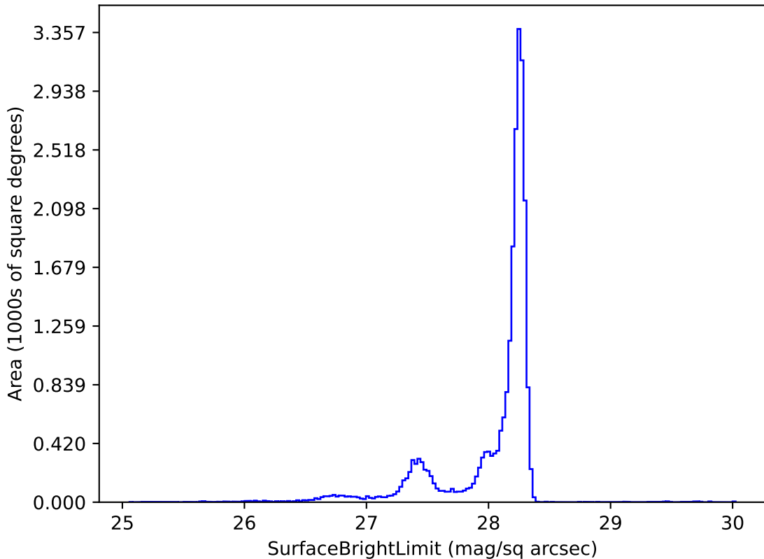
extra_ss_neo5_v3.4_10yrs y: SurfaceBrightLimit
