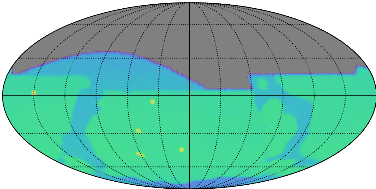
extra_ss_neo5_v3.4_10yrs r: SurfaceBrightLimit
