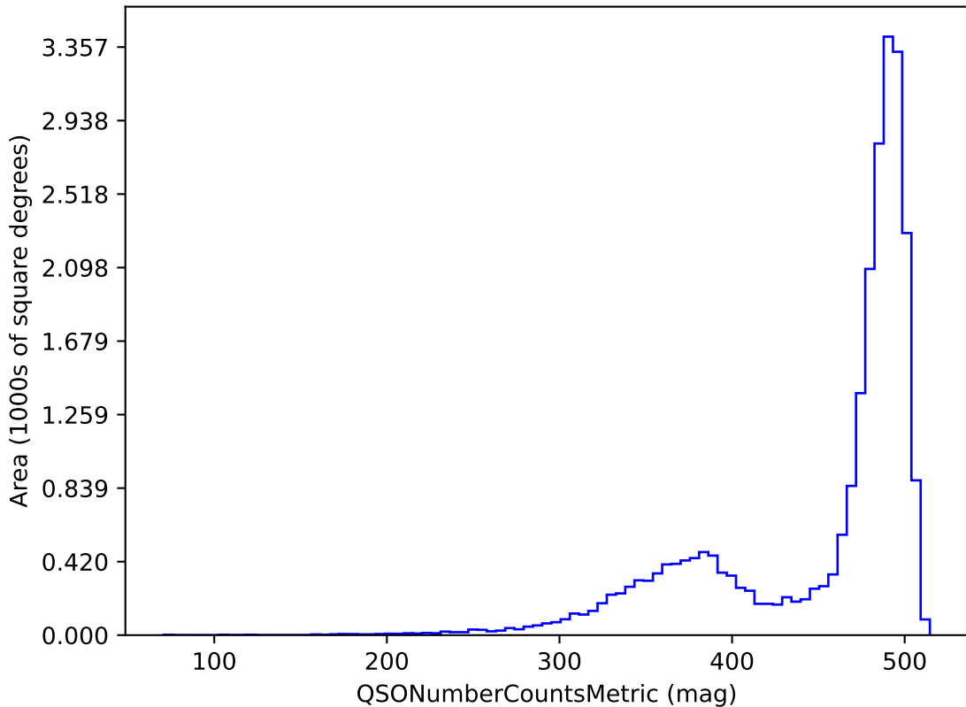
extra_ss_neo5_v3.4_10yrs z band and non-DD: QSONumberCountsMetric
