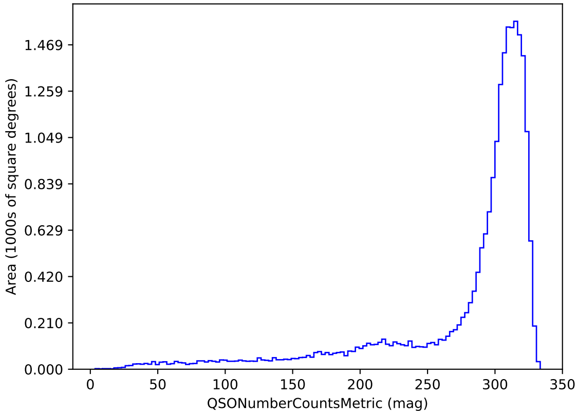
extra_ss_neo5_v3.4_10yrs u band and non-DD: QSONumberCountsMetric
