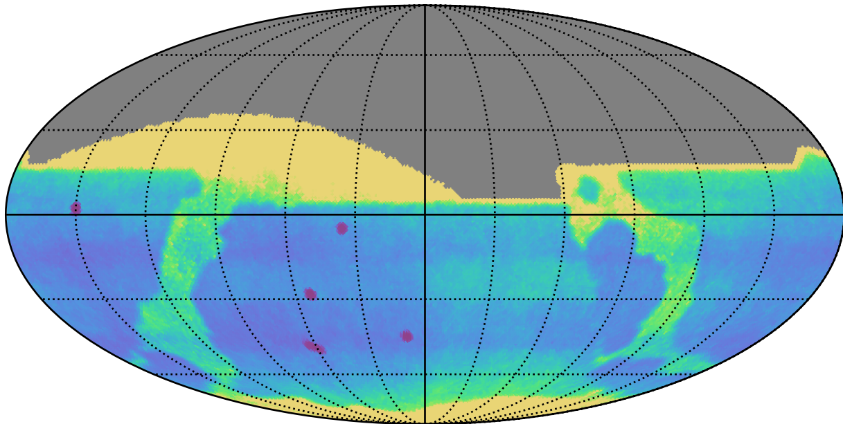
extra_ss_neo5_v3.4_10yrs : Proper Motion Uncert @ 24.0
