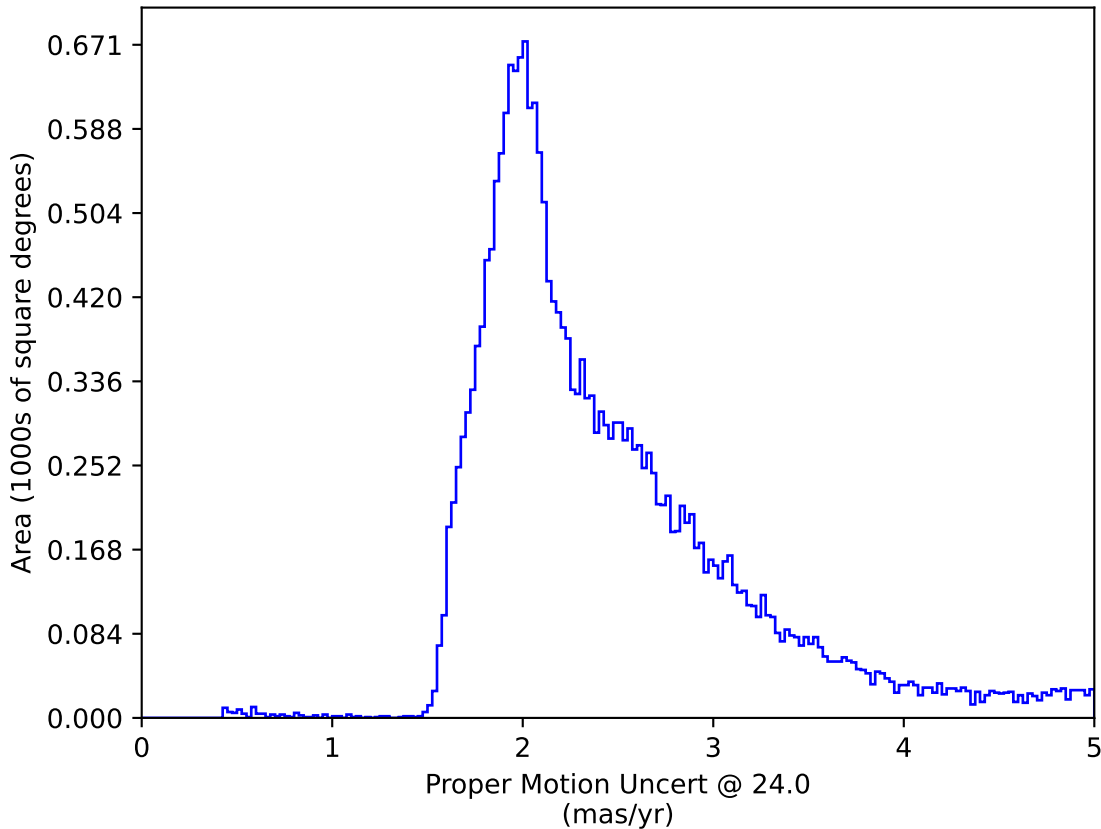
extra_ss_neo5_v3.4_10yrs : Proper Motion Uncert @ 24.0
