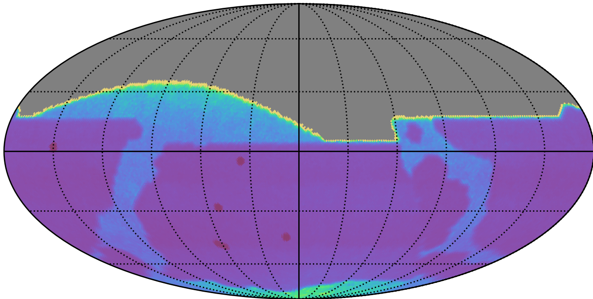
extra_ss_neo5_v3.4_10yrs : Proper Motion Uncert @ 20.5
