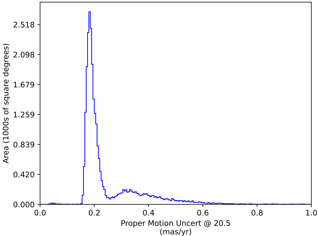
extra_ss_neo5_v3.4_10yrs : Proper Motion Uncert @ 20.5
