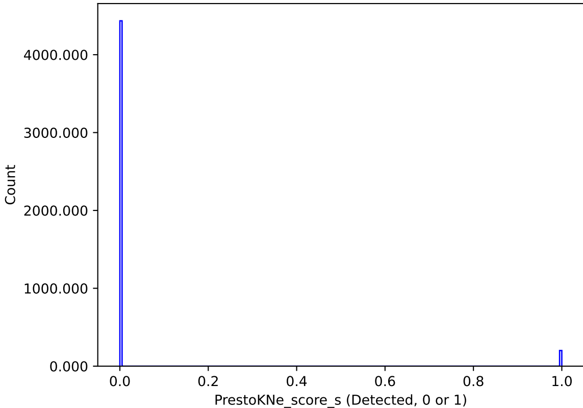
extra_ss_neo5_v3.4_10yrs : PrestoKNe_score_s
