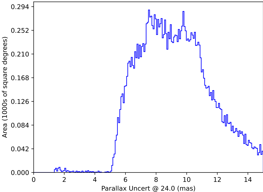
extra_ss_neo5_v3.4_10yrs : Parallax Uncert @ 24.0
