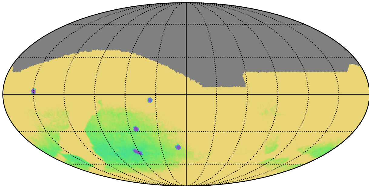
extra_ss_neo5_v3.4_10yrs : Parallax Uncert @ 22.4
