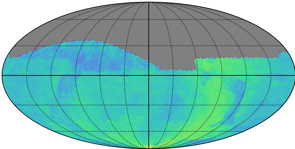
extra_ss_neo5_v3.4_10yrs : Parallax Coverage @ 24.0
