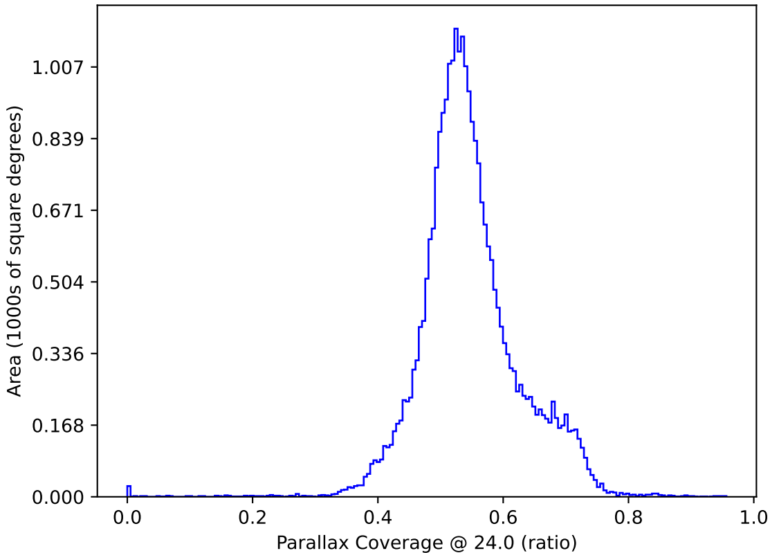
extra_ss_neo5_v3.4_10yrs : Parallax Coverage @ 24.0
