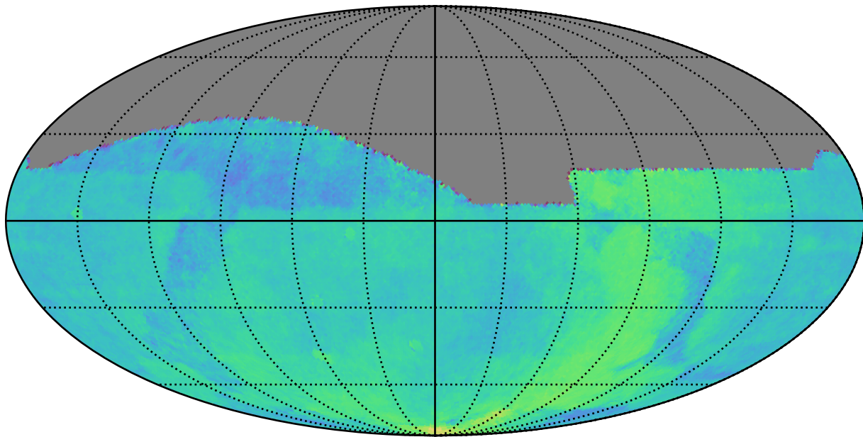
extra_ss_neo5_v3.4_10yrs : Parallax Coverage @ 22.4
