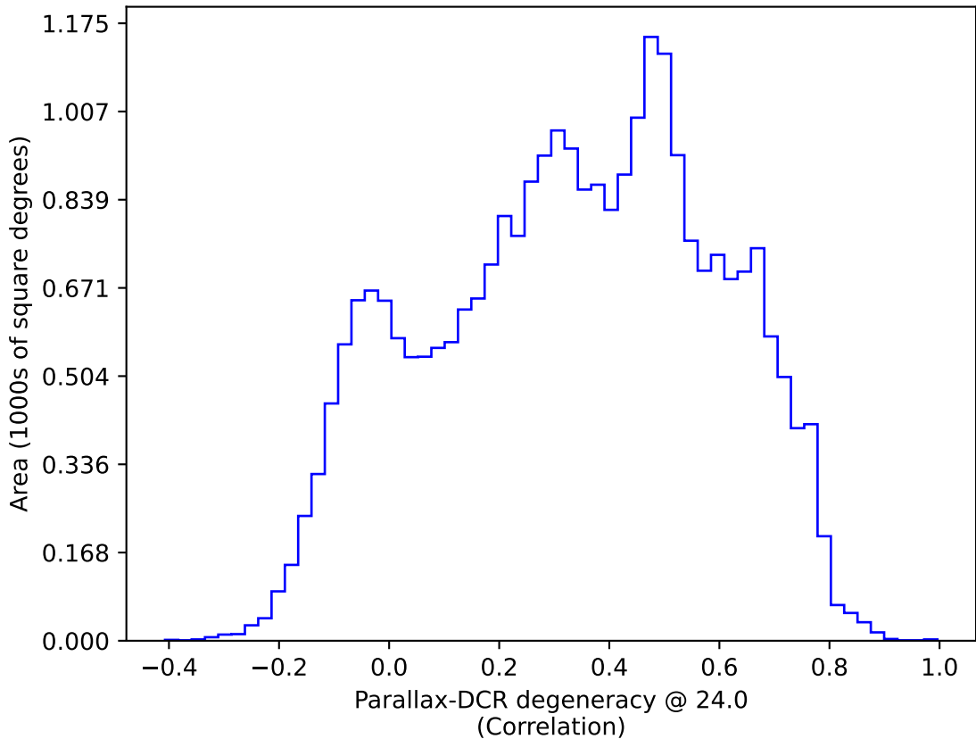
extra_ss_neo5_v3.4_10yrs : Parallax-DCR degeneracy @ 24.0
