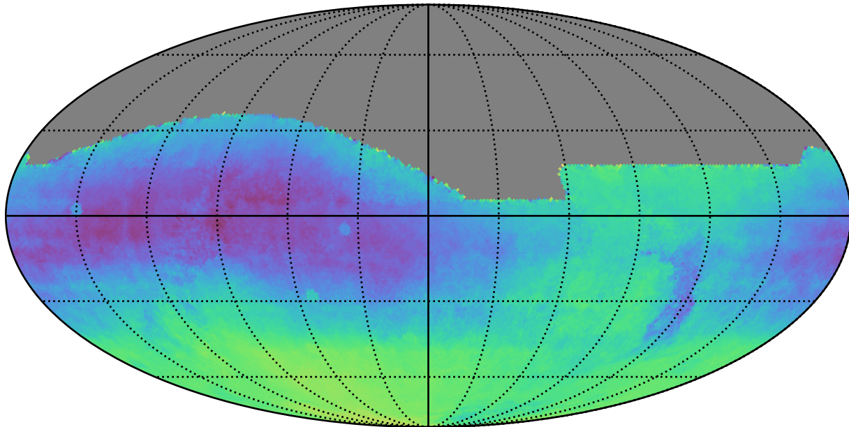
extra_ss_neo5_v3.4_10yrs : Parallax-DCR degeneracy @ 22.4
