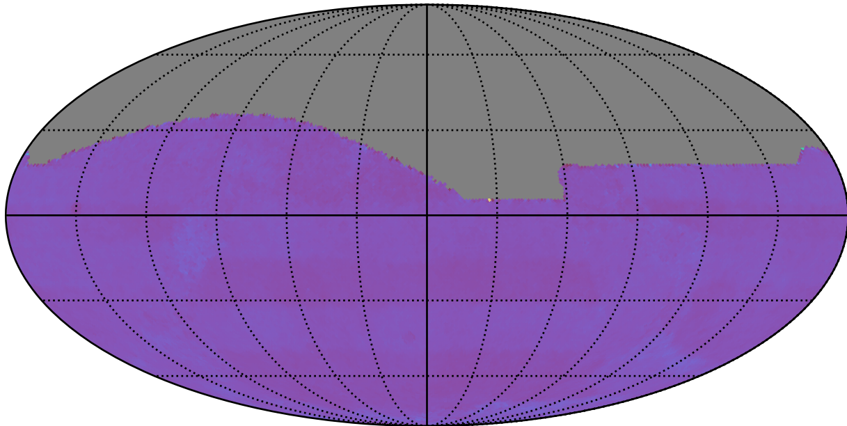
extra_ss_neo5_v3.4_10yrs : Normalized Proper Motion Uncert @ 24.0
