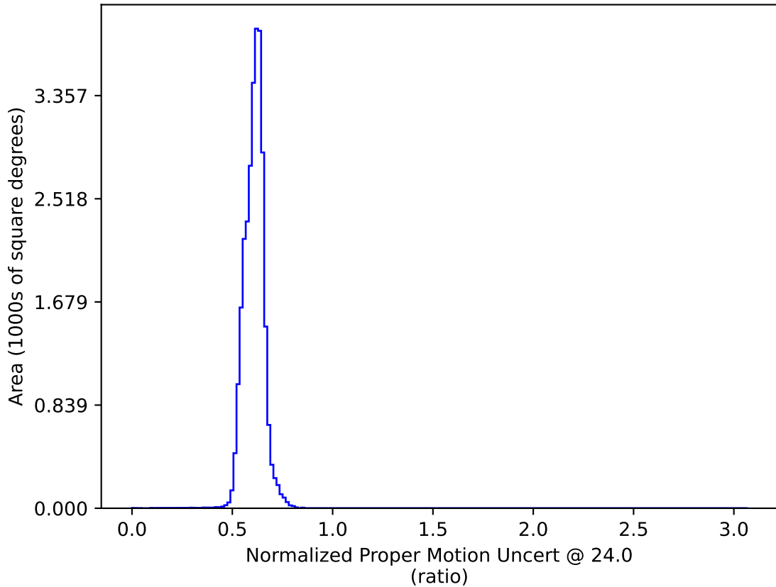
extra_ss_neo5_v3.4_10yrs : Normalized Proper Motion Uncert @ 24.0
