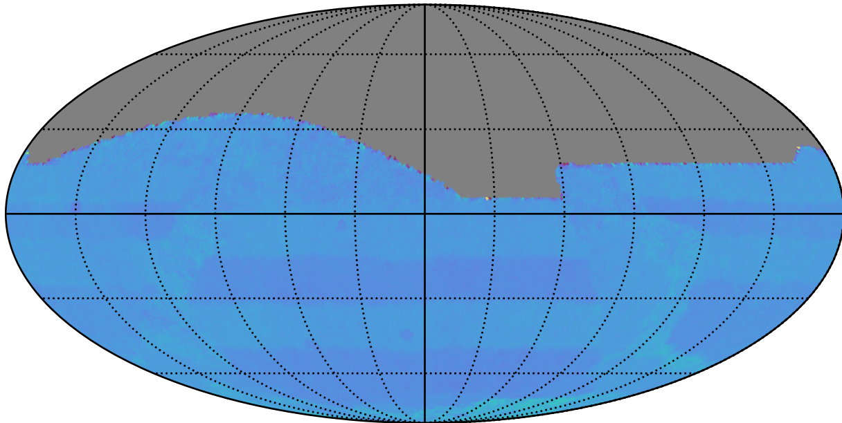
extra_ss_neo5_v3.4_10yrs : Normalized Proper Motion Uncert @ 20.5
