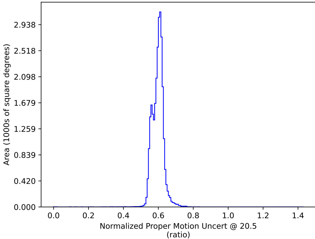
extra_ss_neo5_v3.4_10yrs : Normalized Proper Motion Uncert @ 20.5
