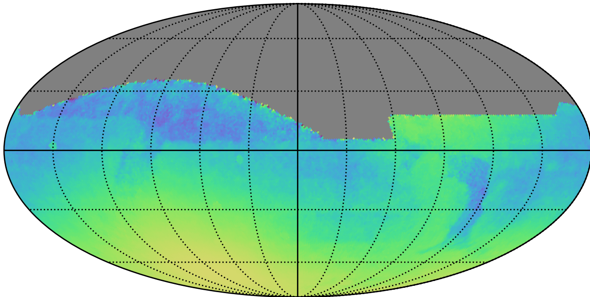
extra_ss_neo5_v3.4_10yrs : Normalized Parallax Uncert @ 24.0
