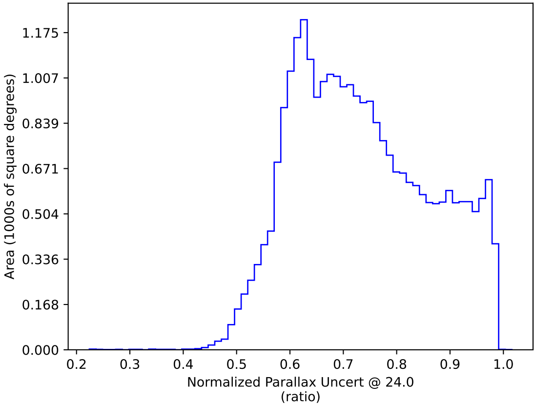
extra_ss_neo5_v3.4_10yrs : Normalized Parallax Uncert @ 24.0
