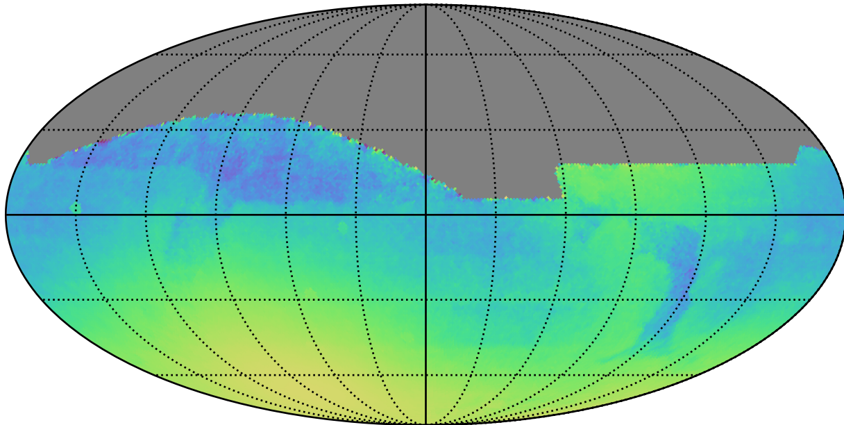
extra_ss_neo5_v3.4_10yrs : Normalized Parallax Uncert @ 22.4
