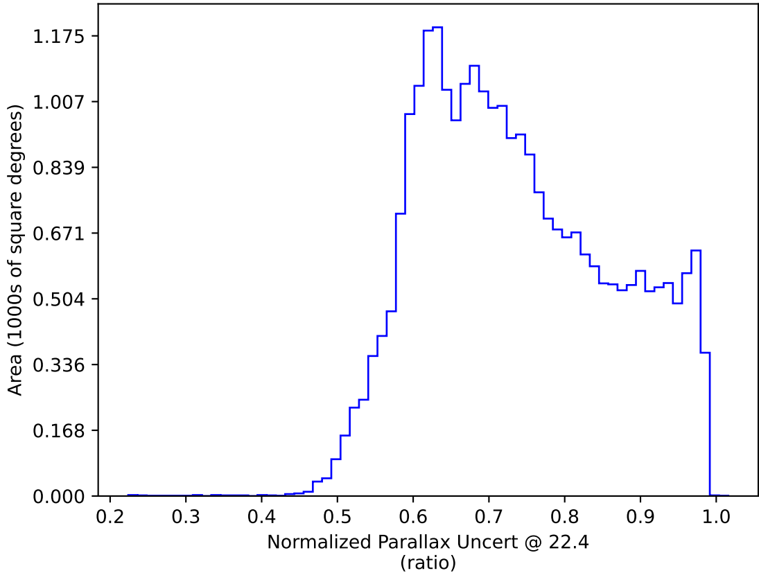
extra_ss_neo5_v3.4_10yrs : Normalized Parallax Uncert @ 22.4
