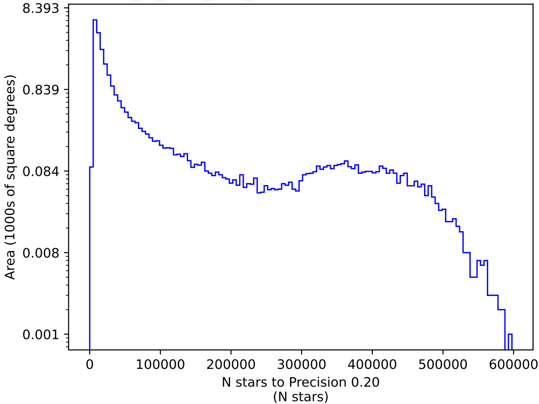
extra_ss_neo5_v3.4_10yrs z: N stars to Precision 0.20
