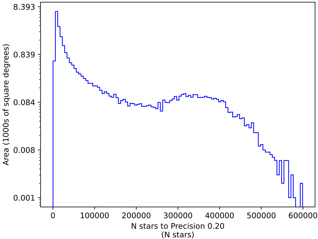
extra_ss_neo5_v3.4_10yrs y: N stars to Precision 0.20
