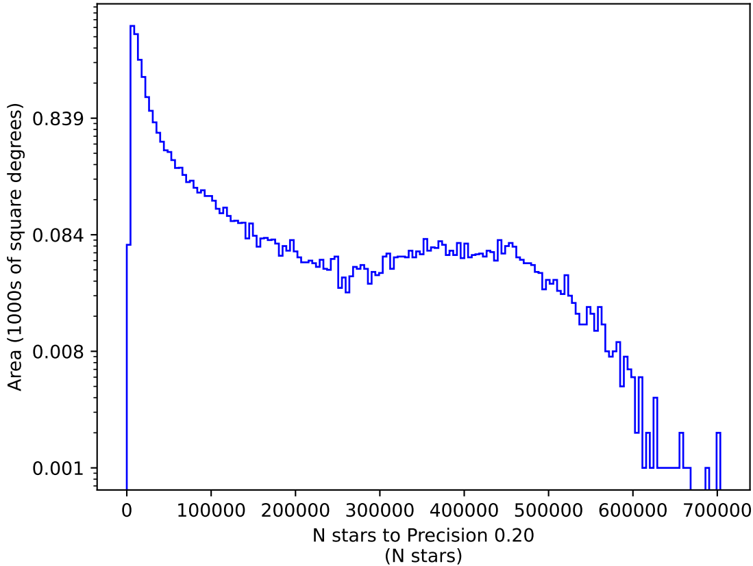
extra_ss_neo5_v3.4_10yrs r: N stars to Precision 0.20
