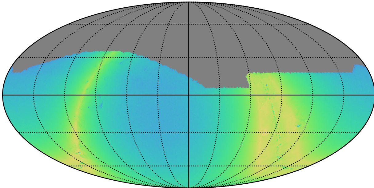
extra_ss_neo5_v3.4_10yrs i: N stars to Precision 0.20
