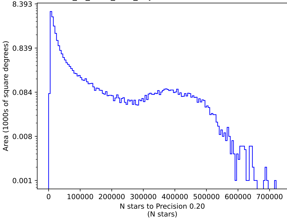
extra_ss_neo5_v3.4_10yrs i: N stars to Precision 0.20
