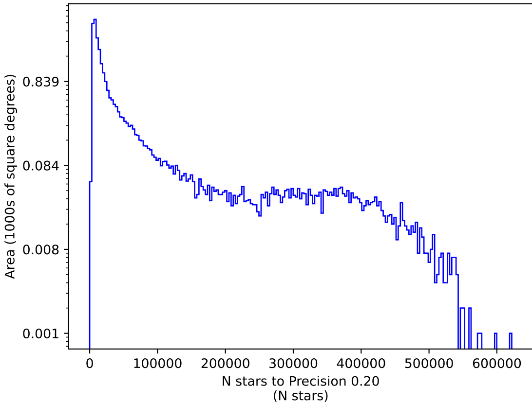
extra_ss_neo5_v3.4_10yrs g: N stars to Precision 0.20
