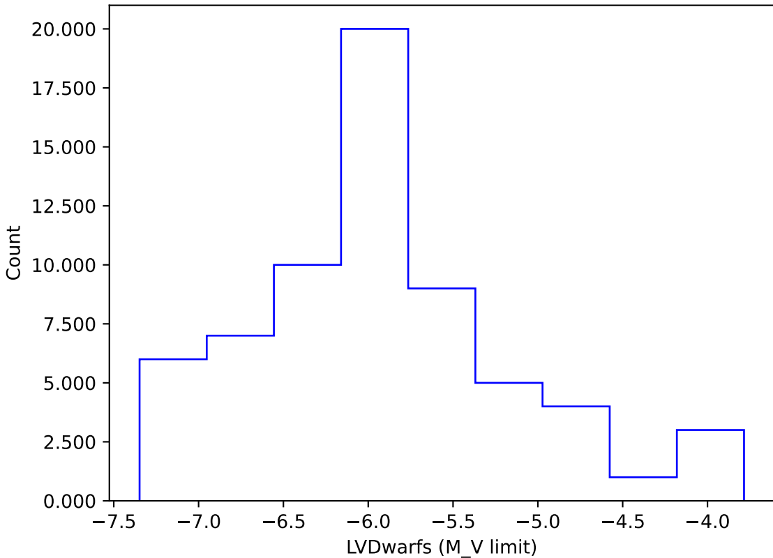
extra_ss_neo5_v3.4_10yrs gi: LVDwarfs
