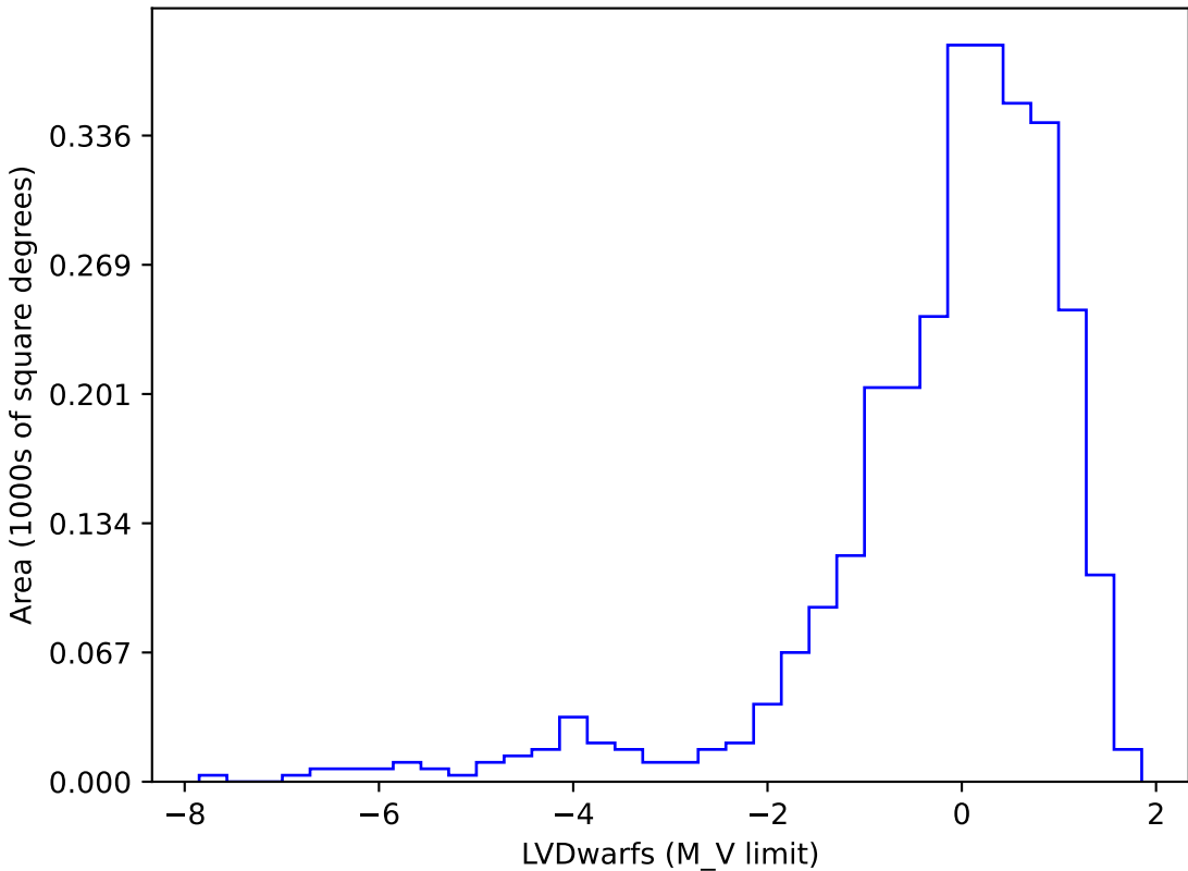
extra_ss_neo5_v3.4_10yrs gi SCP: LVDwarfs
