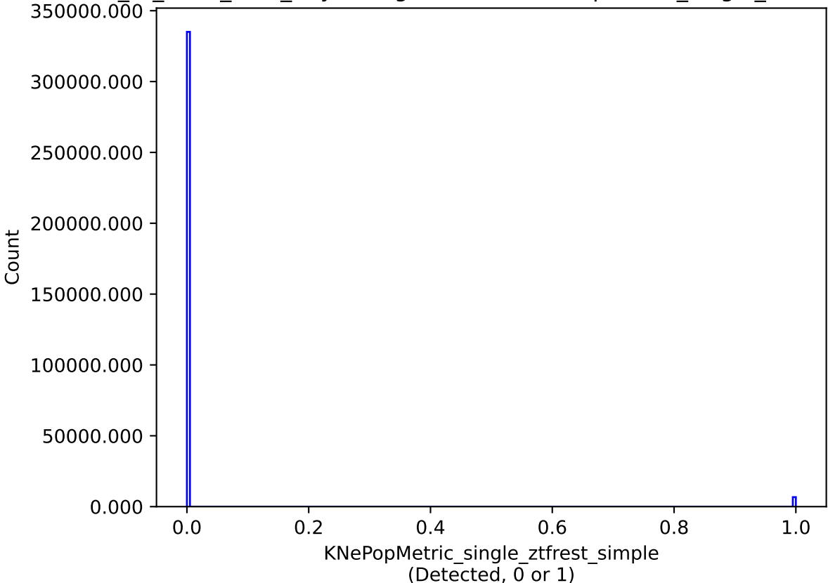
extra_ss_neo5_v3.4_10yrs single model: KNePopMetric_single_ztfrest_simple
