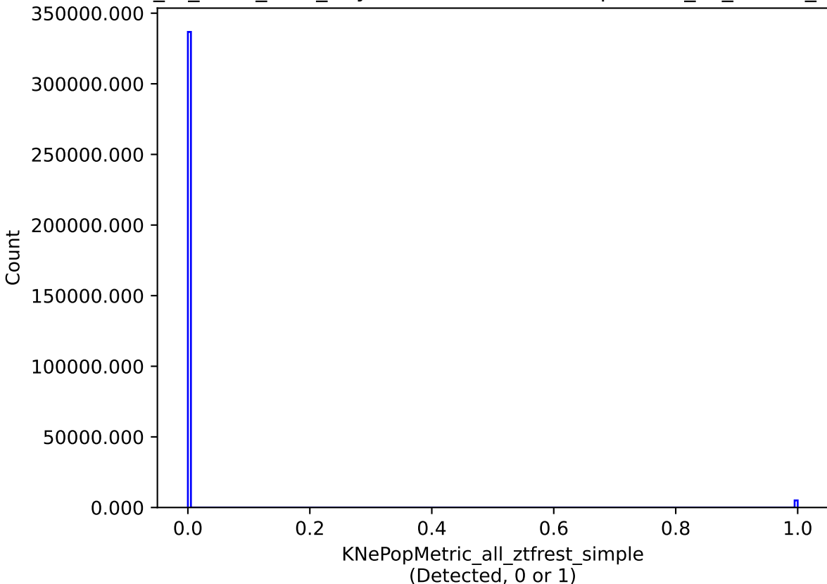
extra_ss_neo5_v3.4_10yrs all models: KNePopMetric_all_ztfrest_simple
